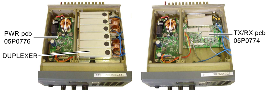
Top cover removed
